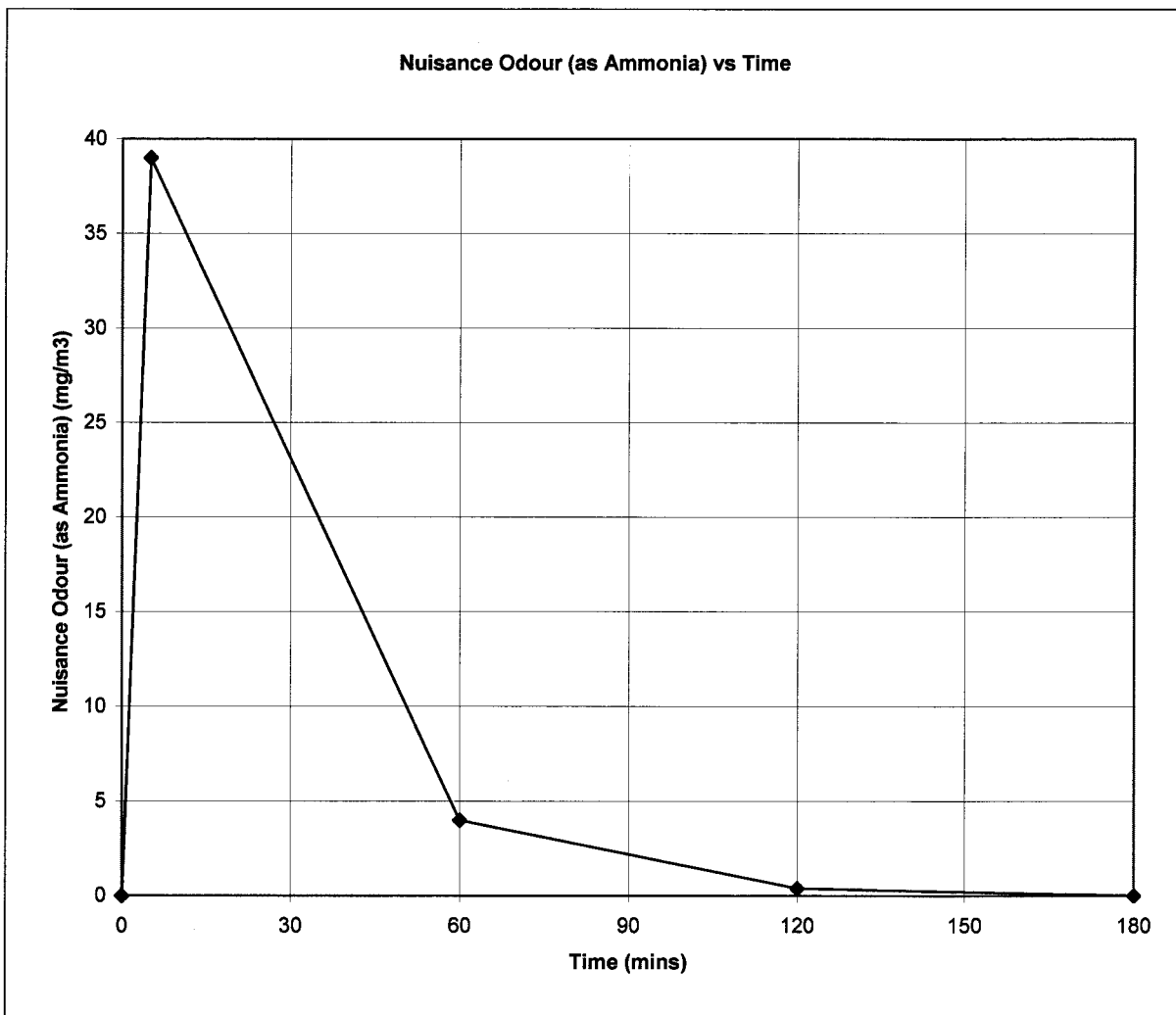
Figure 5: Graph of Nuisance Odour (as Ammonia) Concentration versus Cumulative Time
