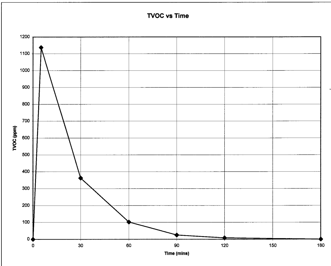
Figure 4: Graph of Total Volatile Organic Compounds Concentration versus Cumulative Time
